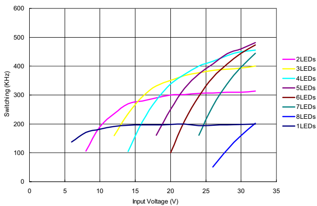
Input Voltage vs Switching Frequency L=47uH
