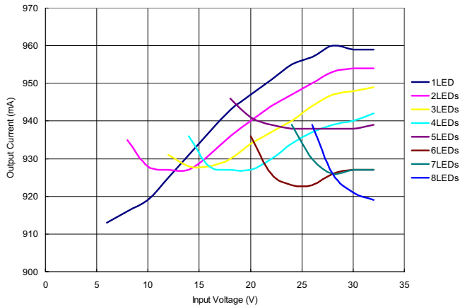
Input Voltage vs Output Current L=47uH
