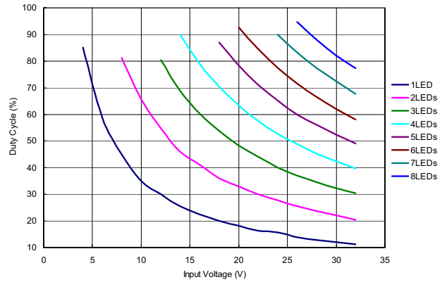
Input Voltage vs Duty Cycle L=47uH
