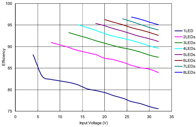
Input Voltage vs Efficiency L=47uH
